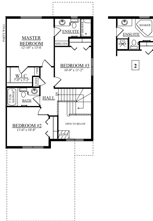
Second Floor 700 sqft
