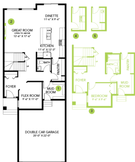
MAIN FLOOR
