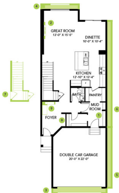
MAIN FLOOR
