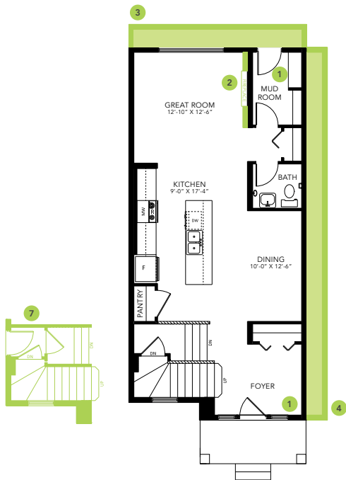
Main Floor 824 SQ FT
