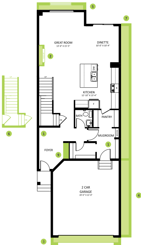
Main Floor 1011 SQ FT
