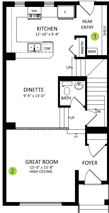
Main Floor 736 SQ FT
