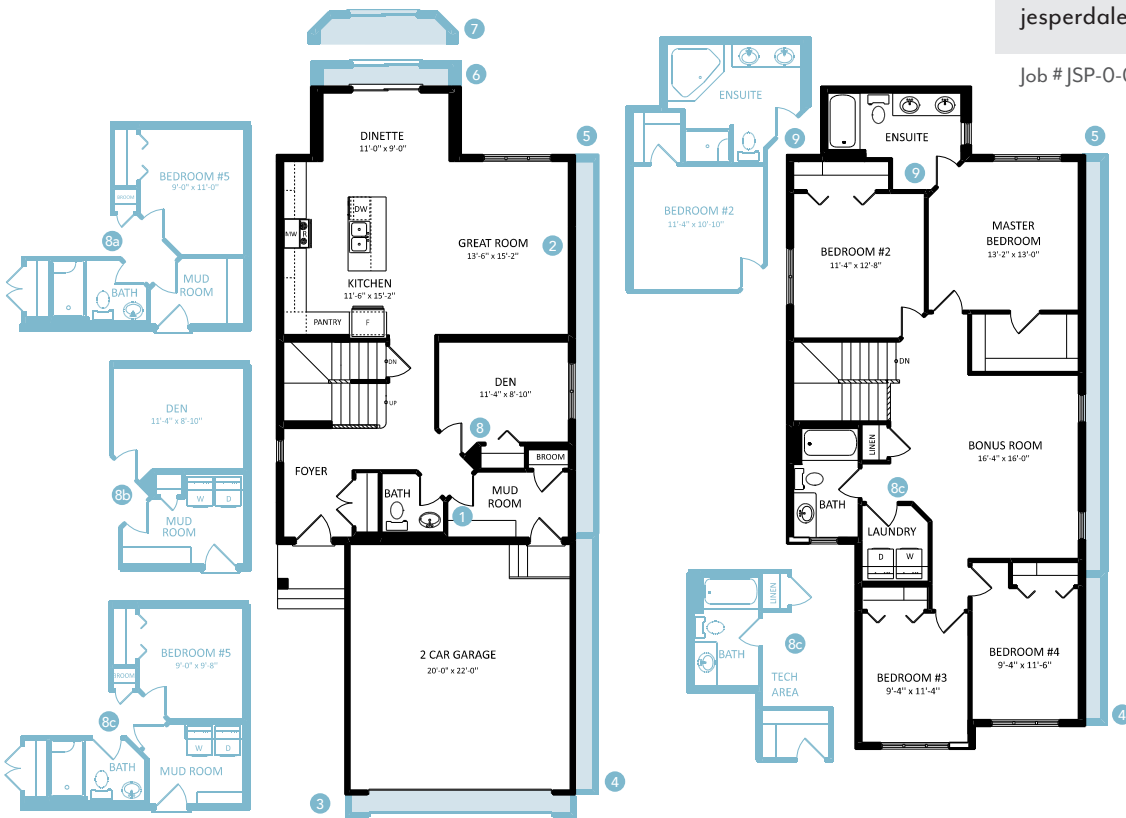
Second Floor 1241 sqft
