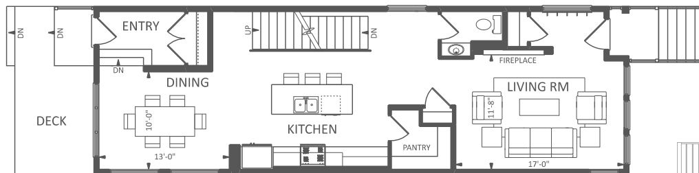
MAIN FLOOR: 908 SQ.FT.
